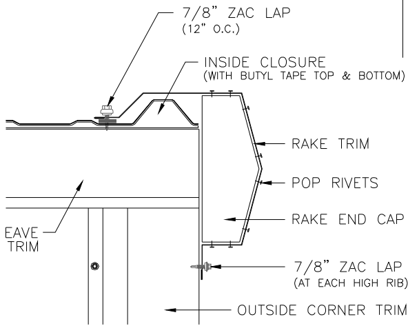
FACE VIEW AT RAKE END CAP
