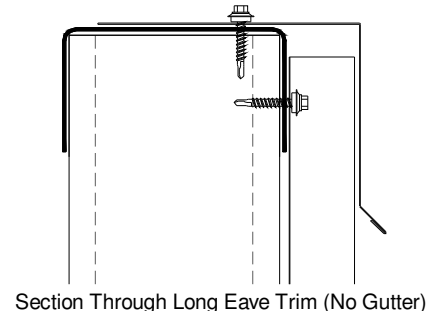
Section Through Long Eave Trim (No Gutter)
