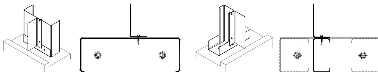
Partition Angle at One Piece Mullion (Sidewall)
