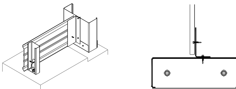
Partition Panel at One Piece Mullion
