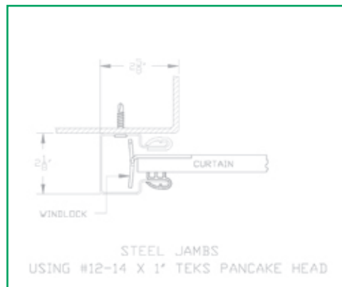
16 GA GUIDE MOUNTING DETAIL (for opening widths over 6'0" through 10'-0")
