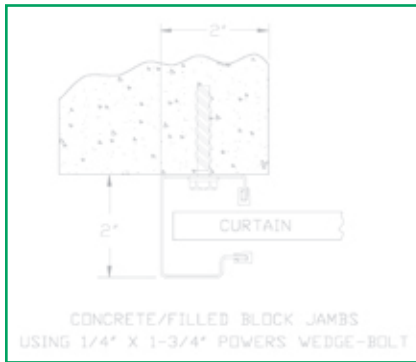
16 GA GUIDE MOUNTING DETAIL (for opening widths over 6'0" through 10'-0")
