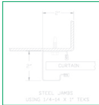
16 GA GUIDE MOUNTING DETAIL (for opening widths over 6'0" through 10'-0")
